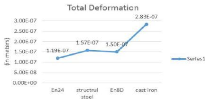
Figure 4: Variation in Total Deformation of Different Materials
