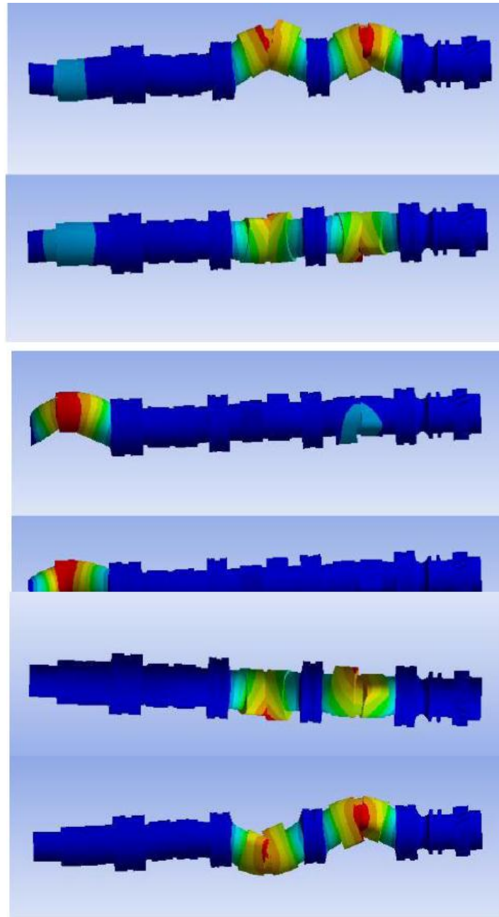
Figure 6: Six Resultant Mode Shape of Camshaft
