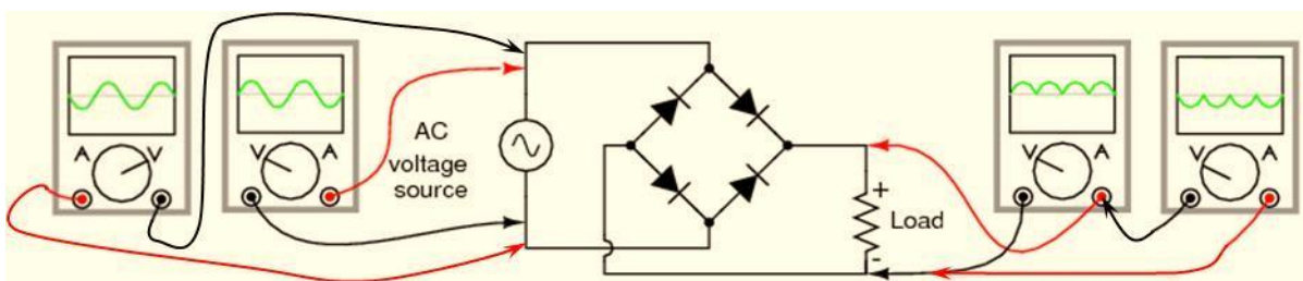
Fig 2.6.8j Bridge Rectifier (secondary utilized voltage = V )
