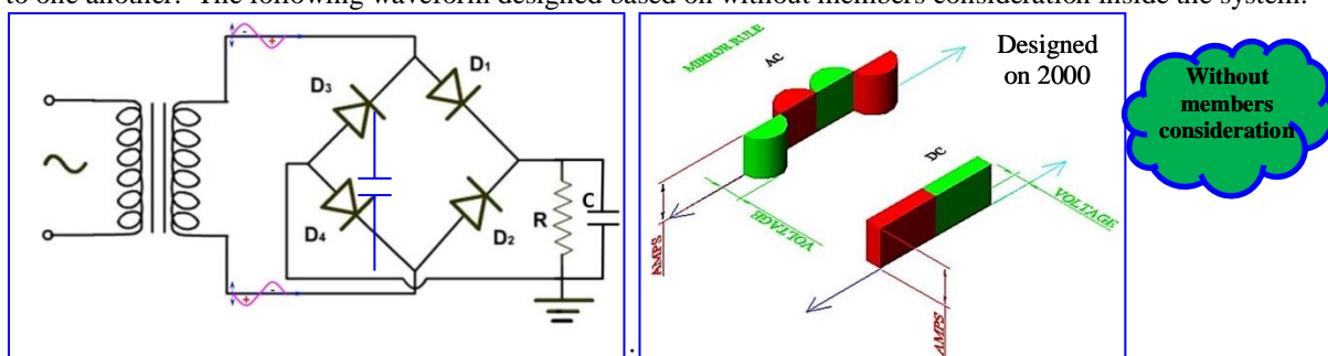
Fig. 2.6.8e AC Transformer with DC converter and graph ("One is opposite to another")
