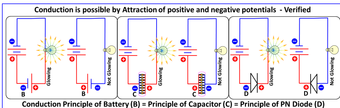
Fig. 2.10e similarity between Battery, Capacitor and PN Diode.
