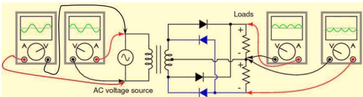
Fig. 2.6.8i Full wave rectifier (secondary voltage = V/2 )
