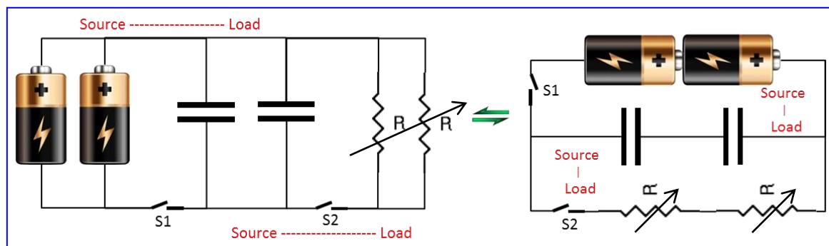
Fig. 2.4.1 Combinations of Capacitor with load under conversion process (charging and discharging)
