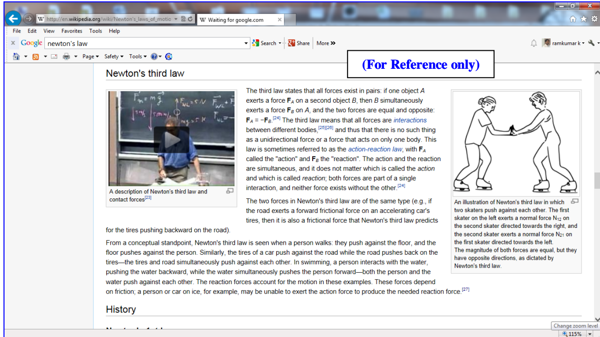
Fig. 2.6.3a Newton’s 3 rd Law taken from Wikipedia for Reference [13]
