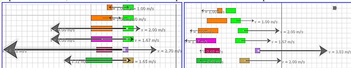
Fig. 2.6.4c Before and after collision of uneven masses (Power is not proportional to Force)
