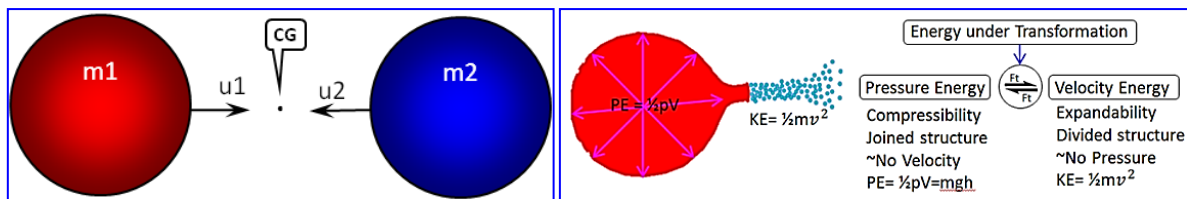
Fig. 2.6.4a Collision of masses (impacting) and its transformation and PE \rightleftharpoons KE
