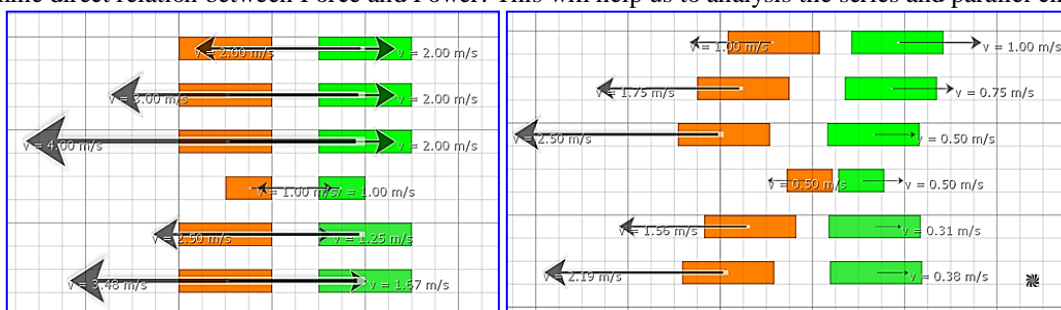
Fig. 2.6.4b Before and after collision of even masses (Power is \propto Force)
