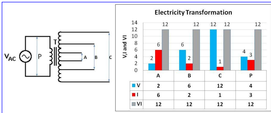
Fig. 2.6a Characteristic Properties of Power Transformer (VI=C) in 2D graph
