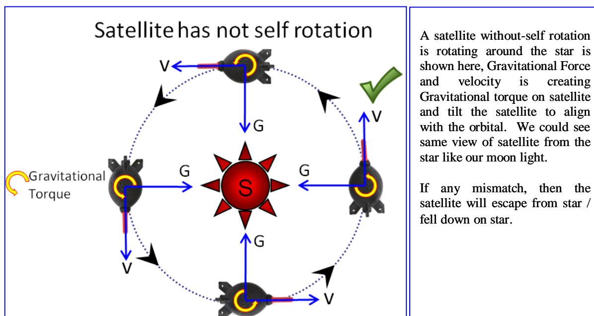
Fig. 2.8.2i Gravitational torque generated by Gravity force and Kinetic Energy
