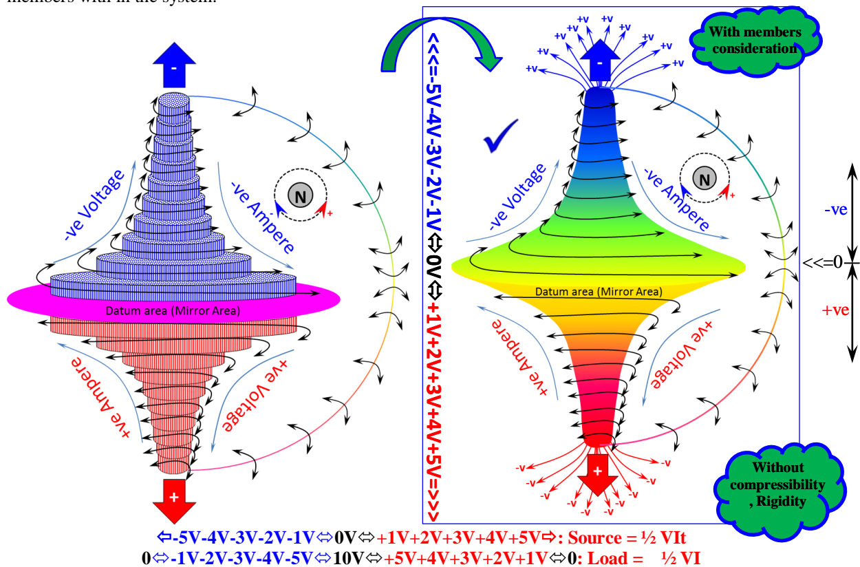
Fig. 2.6.8o Potential Energy ( \frac{1}{2}VI ) with power ( \frac{1}{2}VI ) building Structure with members consideration based on Transformer’s principles, Newton’s 3 rd Law + Mirror rule {Potential Energy with Power Building Structure: Proof: AC Transformer, Series & Parallel combination, Capacitor, ( VI=Constant ), ( VI = Constant ), Electricity polarities, ( V \propto R ), ( I \propto \frac{1}{R} ), ( V \propto \frac{1}{\alpha} I ) and open and short circuits} i.e., (+5V) - (-5V) = 10V (load neutral value) \Rightarrow one number of energy with power is transforming into more number of energy with power.
