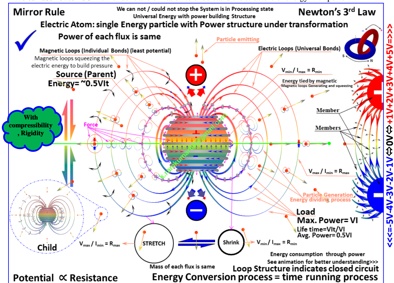
Fig. 2.7c Electric Atom (sectional view) = Electric Energy with power building Structure under transformation (system of time storage with live time running process)
