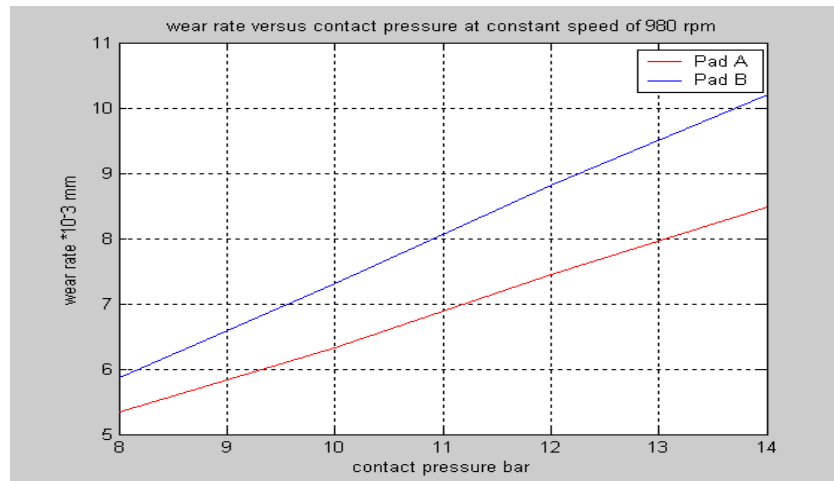
FIGURE 4: WEAR RATE OF TWO BRAKE PAD SAMPLES A AND B PER BRAKE APPLICATION AT A CONSTANT SPEED OF 980RPM.
